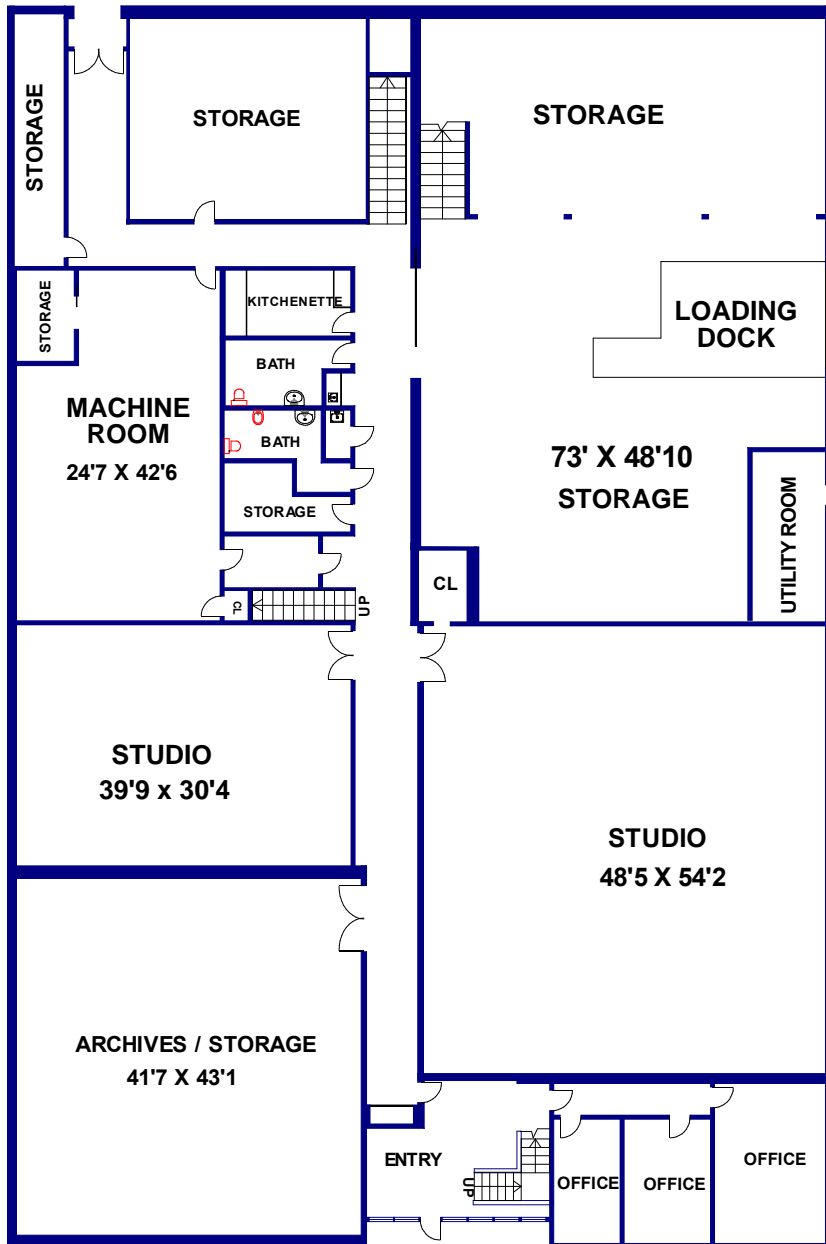
FIRST FLOOR
